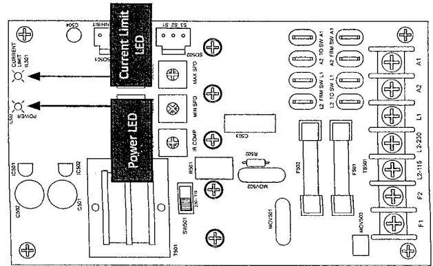
Figure 19. Diagnostic LED Locations
