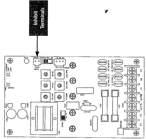
Figure 9. Inhibit Terminals
